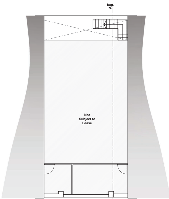
PROPOSED MEZZANINE FLOOR PLAN (ARCH 145)
